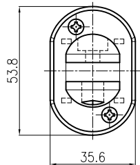
⑤ Z矢視 (S=1/1)
