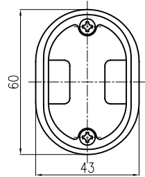
④ Z矢視 (S=1/1)
